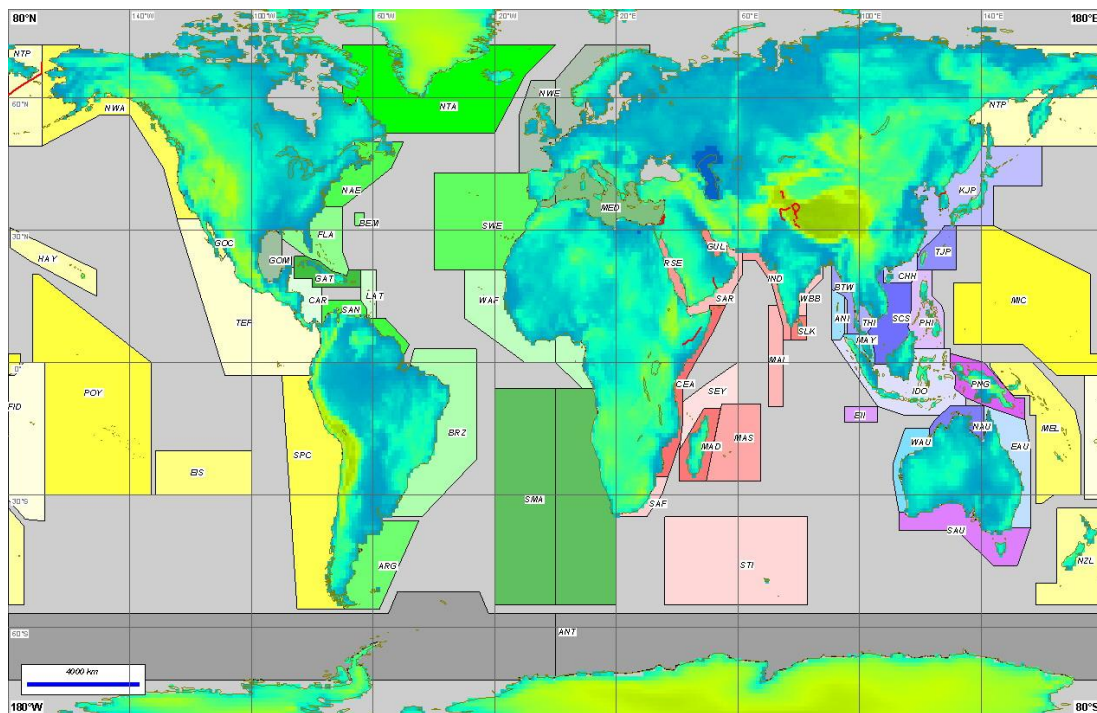
Figure 2.16. A possible classification of marine areas following Hanske & Löser (2006).
